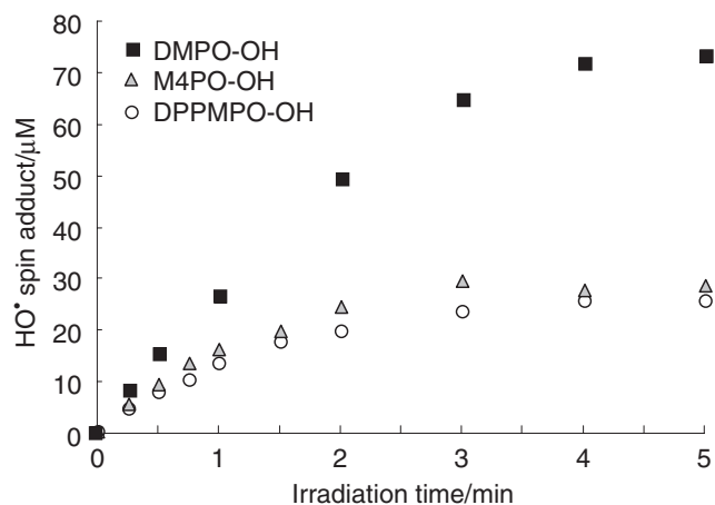
Figure 6. Relationship between spin adducts formation and ultrasound irradiation time. Each spin trap agent was used at their optimal concentration, i.e., 300 mM for DMPO and M4PO, and 20 mM for DPPMPO. Although spin adduct of hydroxyl radical increased with irradiation time, the amount of hydroxyl radical trapped by M4PO and DPPMPO was less than half of that trapped by DMPO. Each value represents the mean of duplicate determinations.
