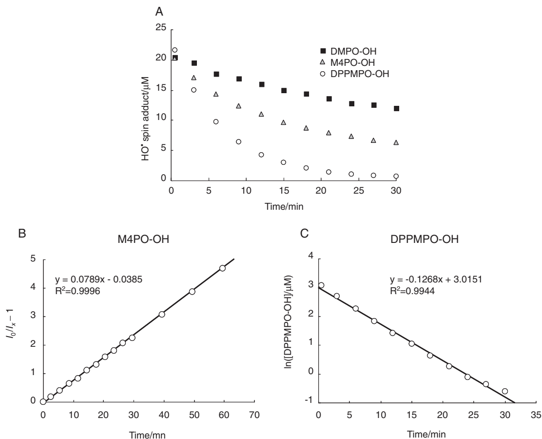
Figure 7. Analysis of decay curve of 20\text{ }\mu\text{M} spin adduct of hydroxyl radical. (A) DMPO-OH was the most stable followed by M4PO-OH and DPPMPO-OH. The half-lives of DMPO-OH, M4PO-OH, and DPPMPO-OH were 41.8, 12.7, and 5.5 min, respectively. (B) M4PO-OH decayed in inverse proportion to time suggesting second-order reaction. The inverse proportion was linearized by the equation I_0/I_x - 1 = ax + b , where I_0 is the initial concentration of M4PO-OH and I_x is the concentration of M4PO-OH at each time interval. (C) On the other hand, since plots of natural logarithm of DPPMPO-OH against time showed a linear relationship, it was suggested that DPPMPO-OH decayed by first-order reaction. Each value represents the mean of duplicate determinations.
