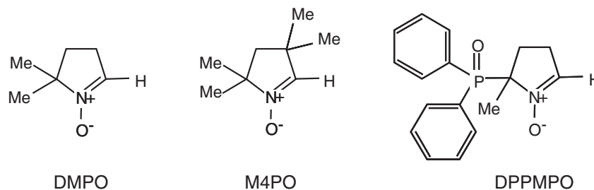
Figure 8. Structures of DMPO, M4PO, and DPPMPO.
