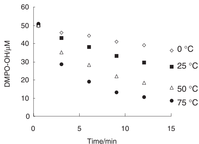
Figure 4. The influence of temperature on the decay curve of DMPO-OH. The half-life decreased with the increase of temperature. Each value represents the mean of triplicate determinations.
