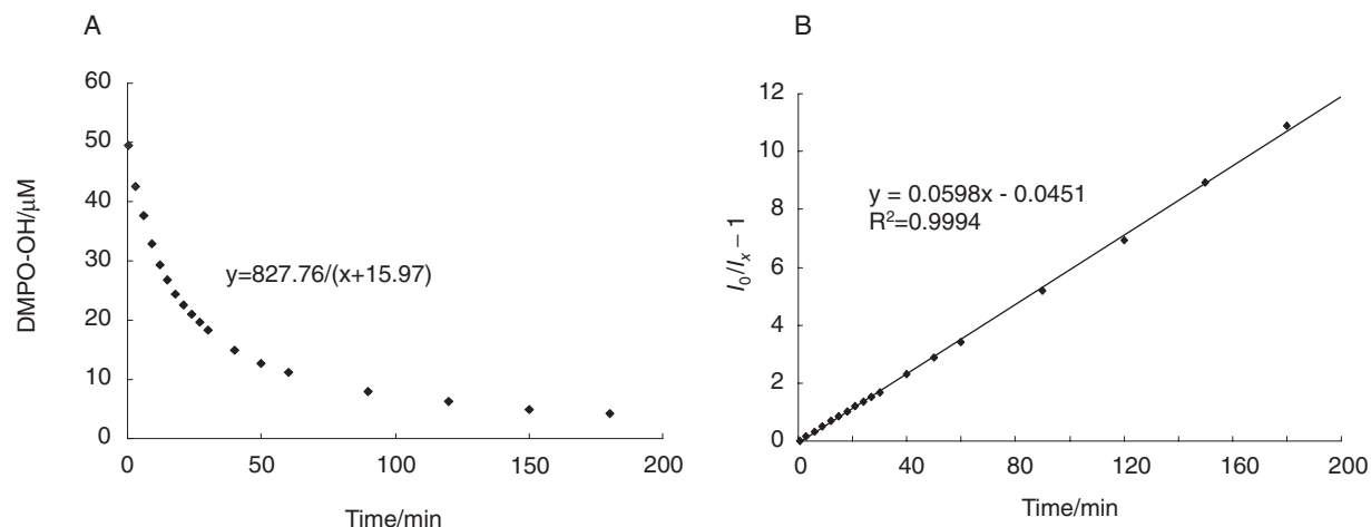
Figure 3. Decay curve of 50 \mu\text{M} DMPO-OH generated by ultrasound irradiation of ultrapure water. (A) DMPO-OH decreased inversely with time. The half-life was 16.6 min. (B) The inverse proportion was linearized by the equation I_0/I_x - 1 = ax + b , where I_0 is the initial concentration of DMPO-OH and I_x is the concentration of DMPO-OH at each time interval. Each value represents the mean of triplicate determinations.
