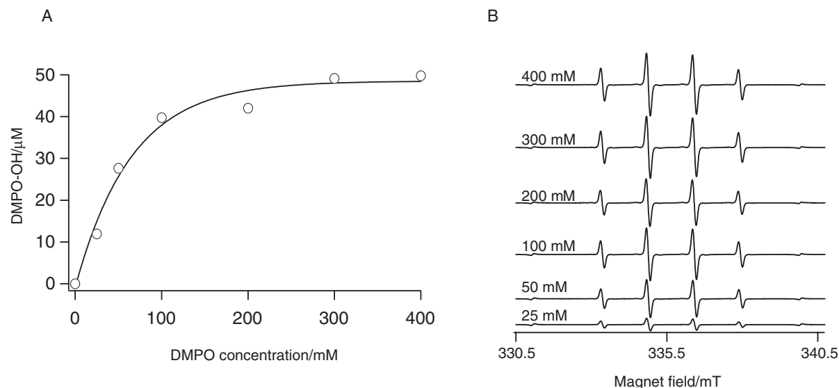
Figure 1. Saturation curve of DMPO-OH. (A) DMPO-OH increased with the concentration of DMPO and then was saturated. (B) The representative ESR spectrum of DMPO-OH generated at different concentrations of DMPO. Each value in Figure 1A represents the mean of triplicate determinations.
