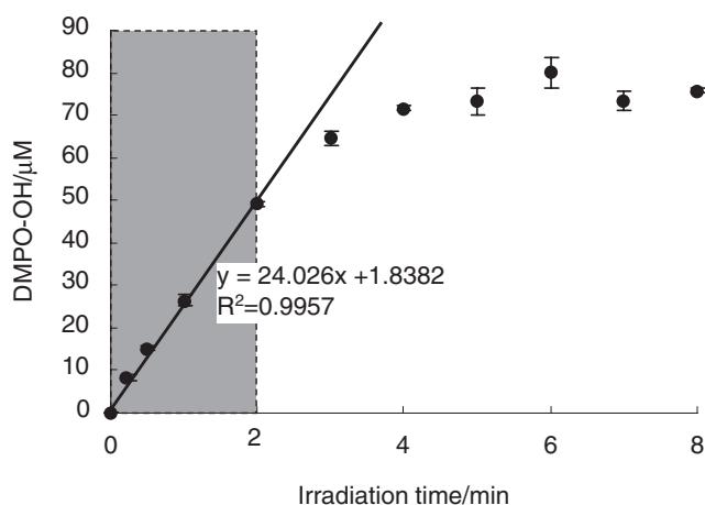
Figure 2. Saturation curve of DMPO-OH formation versus ultrasound irradiation time. DMPO-OH increased linearly up to 2 min with high correlation coefficient of over 0.997. Then, DMPO-OH was gradually saturated with the increase of irradiation time. Each value represents the mean of triplicate determinations with standard deviation.
