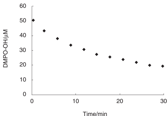
Figure 5. Decay curve of 50 \mu\text{M} DMPO-OH generated by laser irradiation of 1 M \text{H}_2\text{O}_2 . DMPO-OH decreased inversely with time and the half-life almost corresponded to that of 50 \mu\text{M} DMPO-OH generated by ultrasound irradiation of ultrapure water. Each value represents the mean of duplicate determinations.
